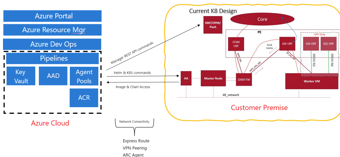
Figure 1-1 PADS High Level Architecture
